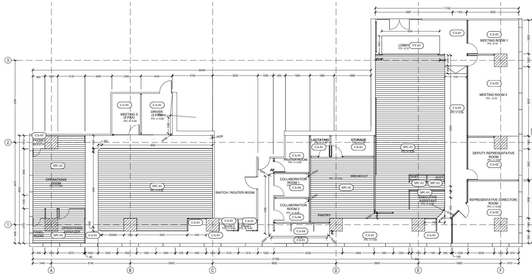
INT-102 FLOOR FINISH PLAN SCALE 1 : 150
