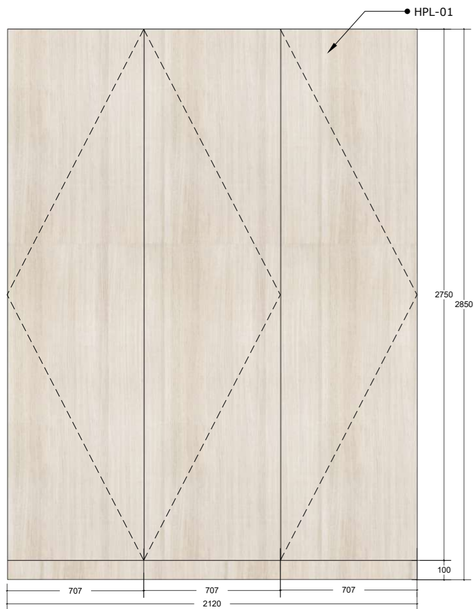
03 FRONT VIEW INT-513 Scale: 1:20
