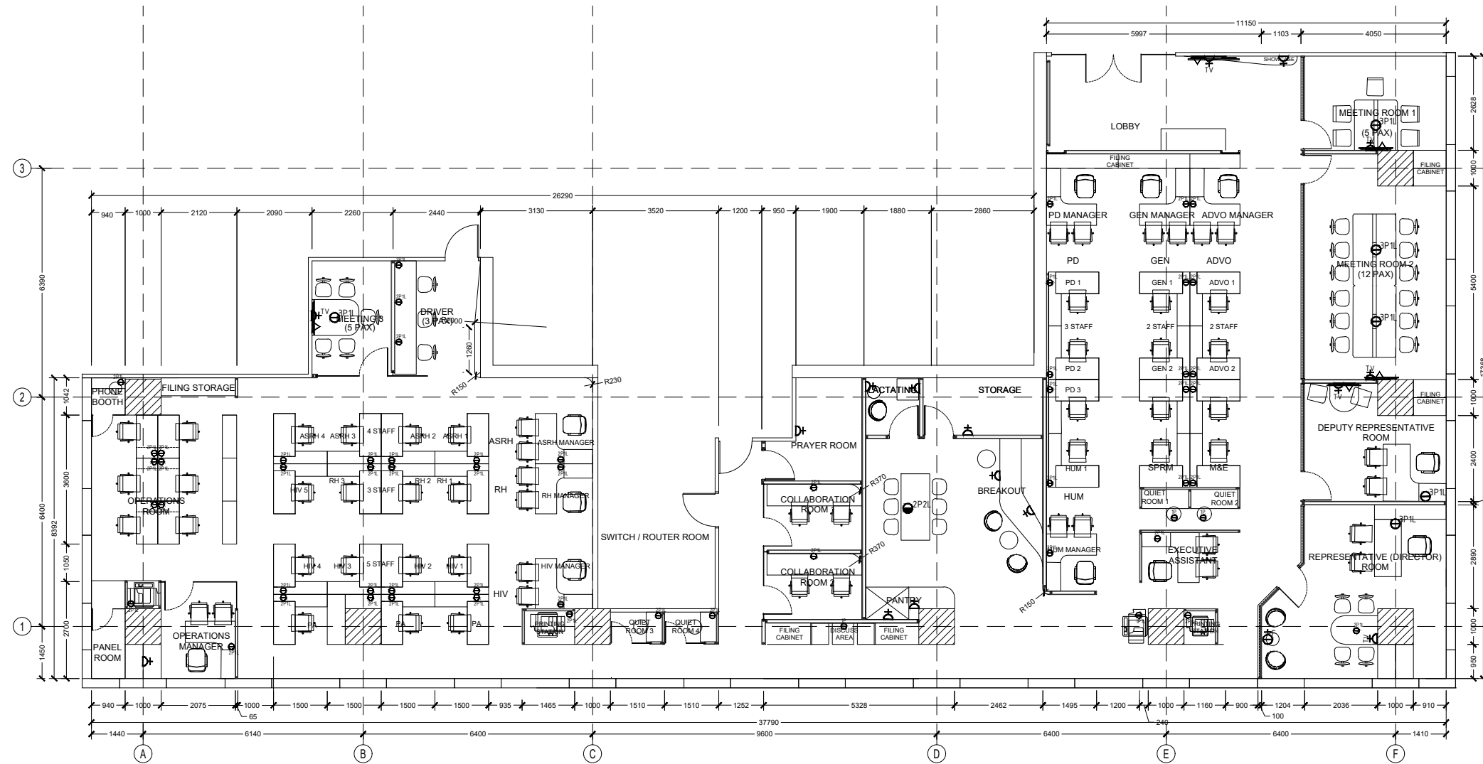
INT-109 LAN & POWER OUTLET PLAN SCALE 1 : 150
