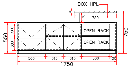
VIEW SIDE CREDENZA
