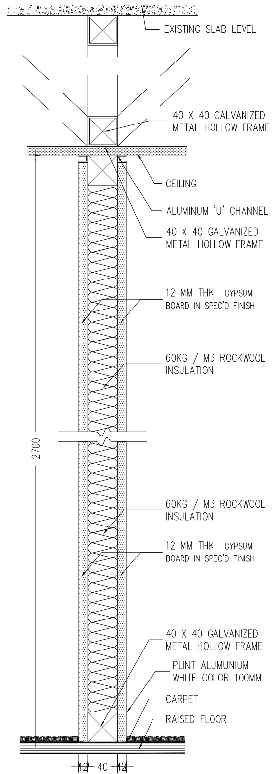
2 DETAIL PARTITION WG2 INT-301 SCALE 1:5
