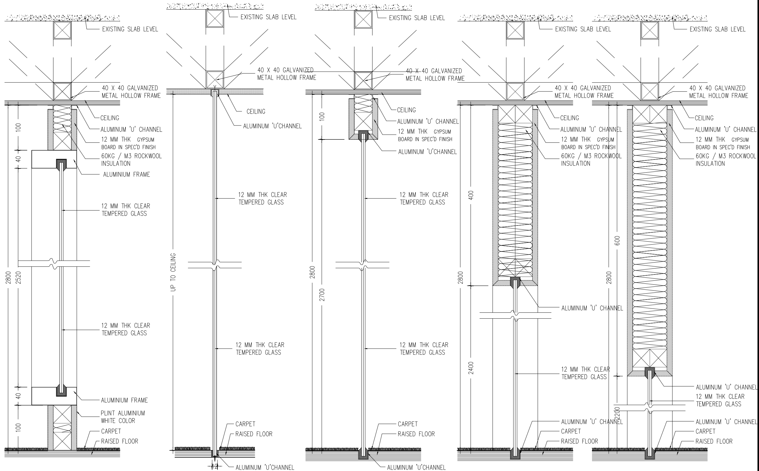
1 DETAIL PARTITION WT1 INT-303 SCALE 1:5
