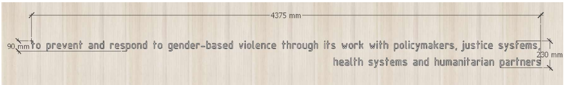
03 INT-600 DETAIL LETTERING QUOTE ( WALL FINISH WORK D9)
