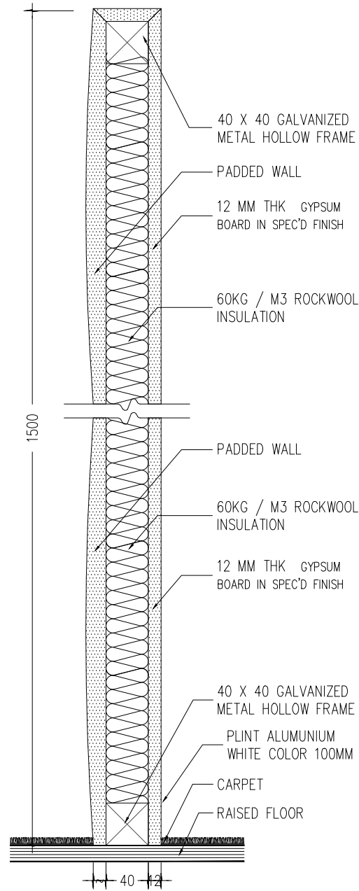
1 DETAIL PARTITION WG4 INT-302 SCALE 1:5
