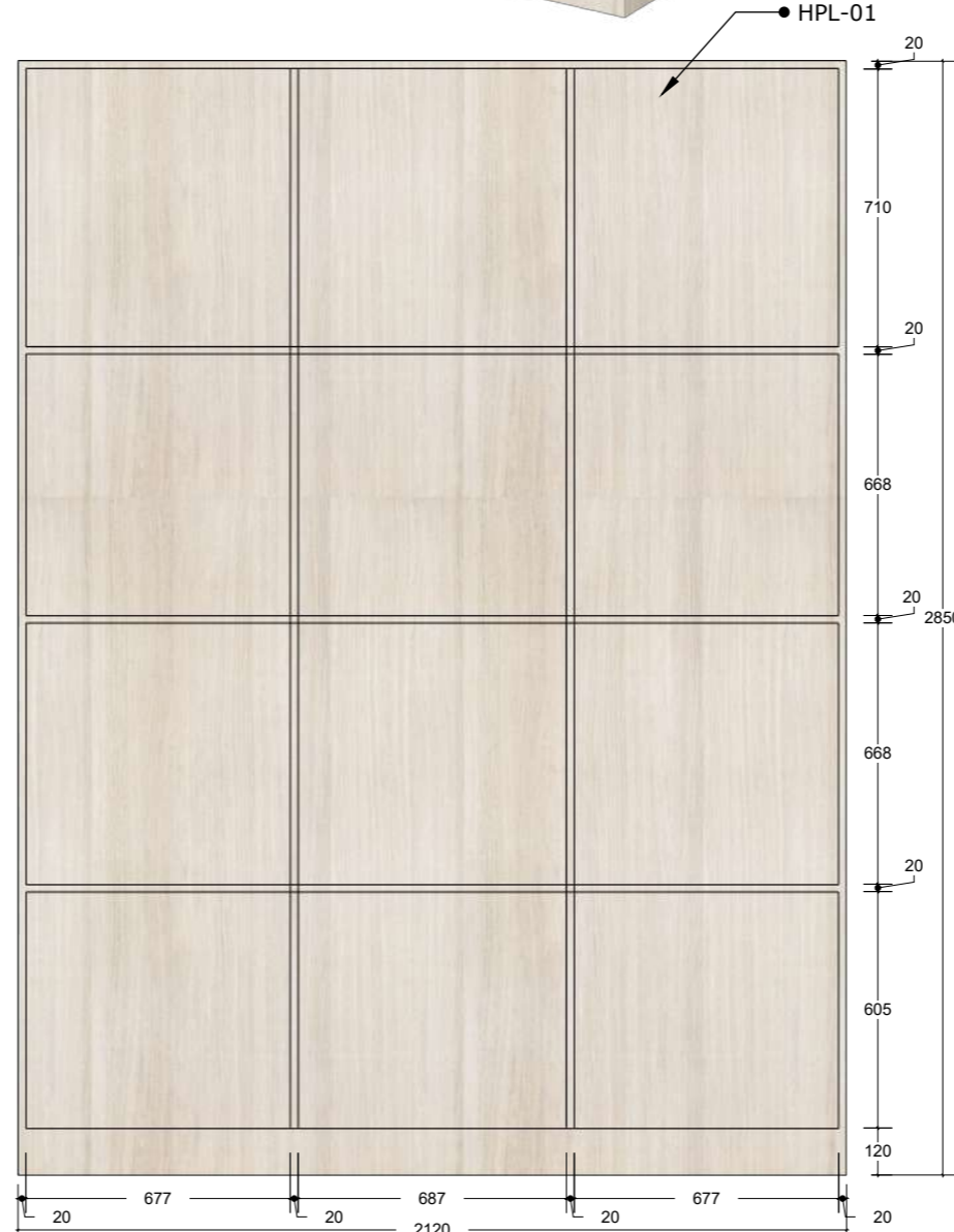
04 FRONT VIEW WITHOUT DOOR INT-513 Scale: 1:20
