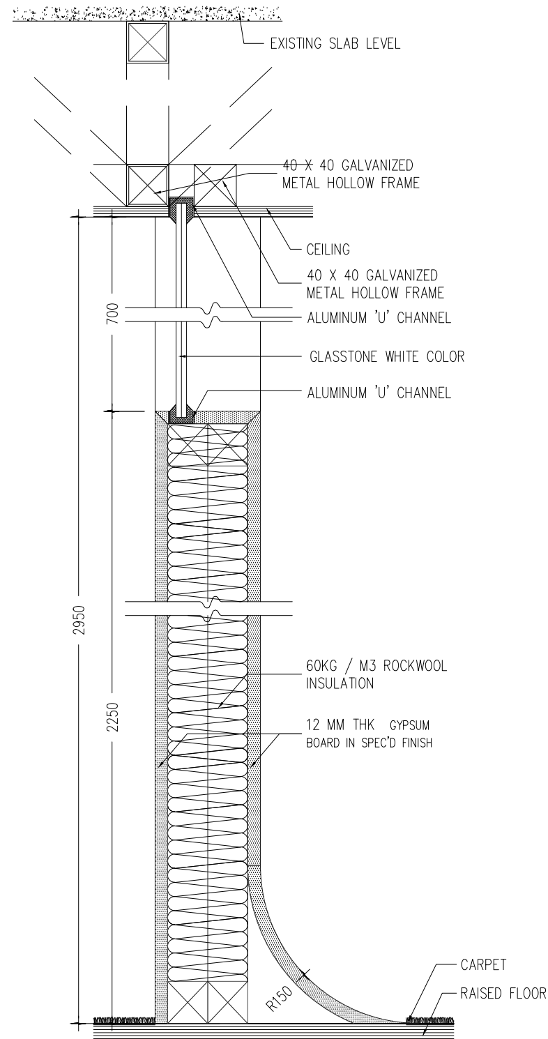
2 DETAIL PARTITION WG5 INT-302 SCALE 1:5
