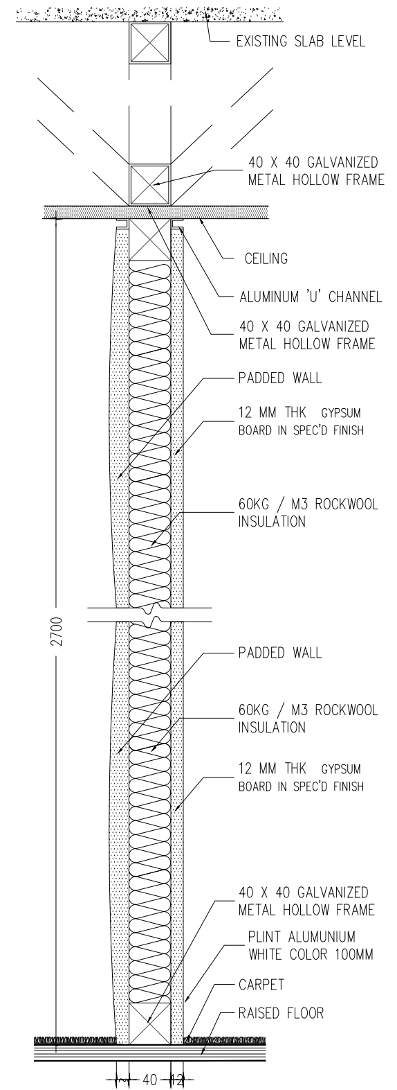
3 DETAIL PARTITION WG3 INT-301 SCALE 1:5
