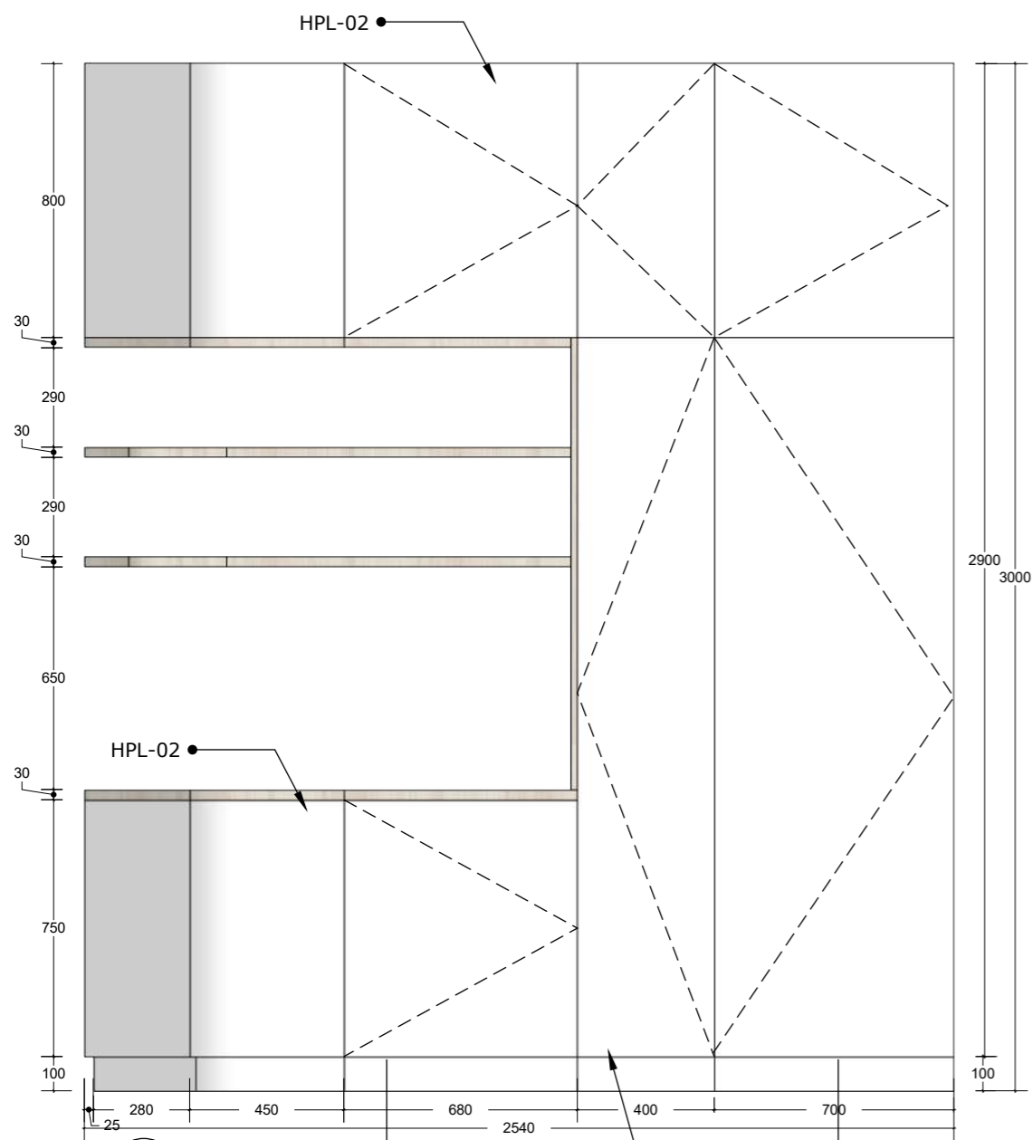
03 FRONT VIEW INT-509 Scale: 1:20
