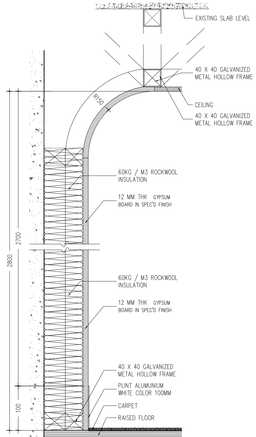
3 DETAIL PARTITION WG6 INT-302 SCALE 1:5
