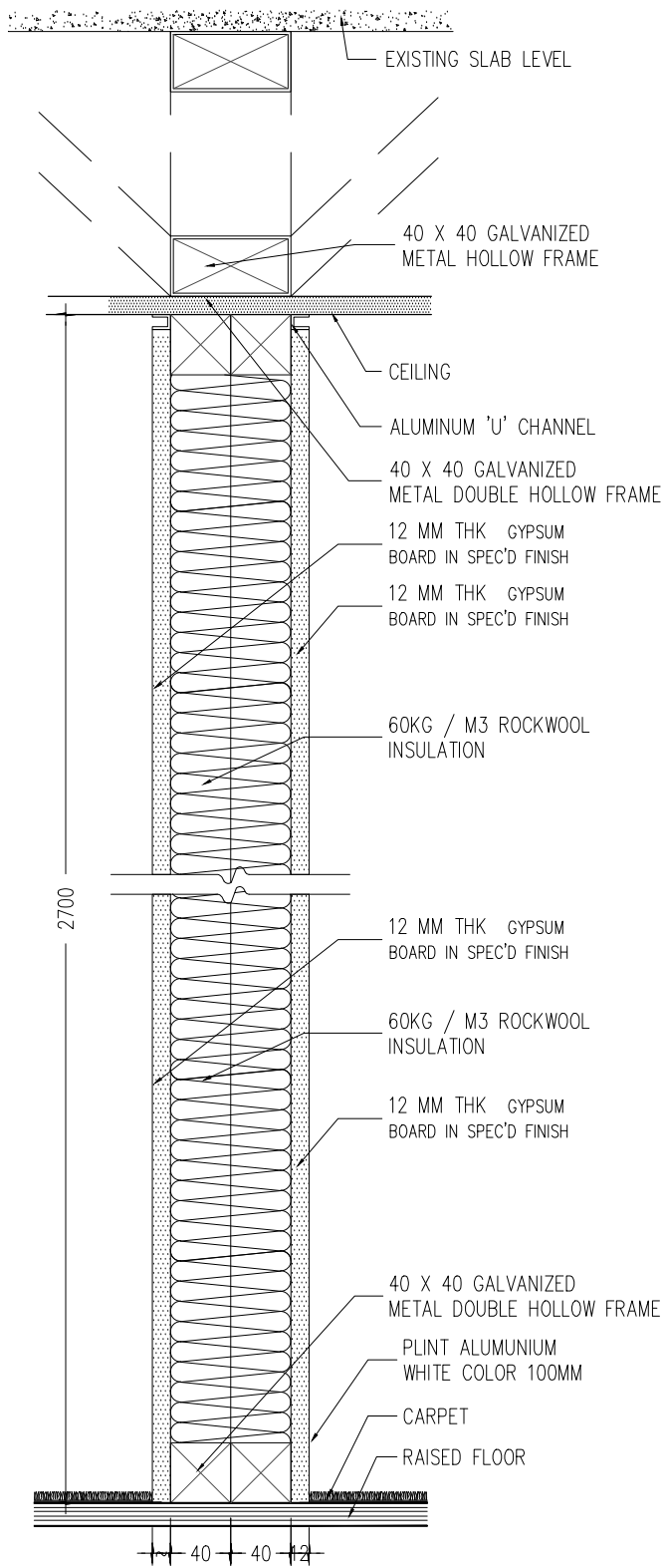
1 DETAIL PARTITION WG1 INT-301 SCALE 1:5
