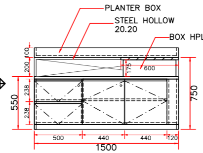
VIEW SIDE CREDENZA
