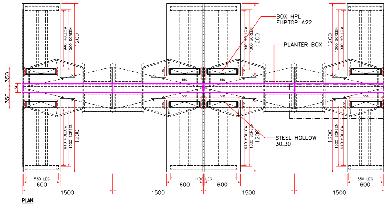
TOP VIEW INT-518
