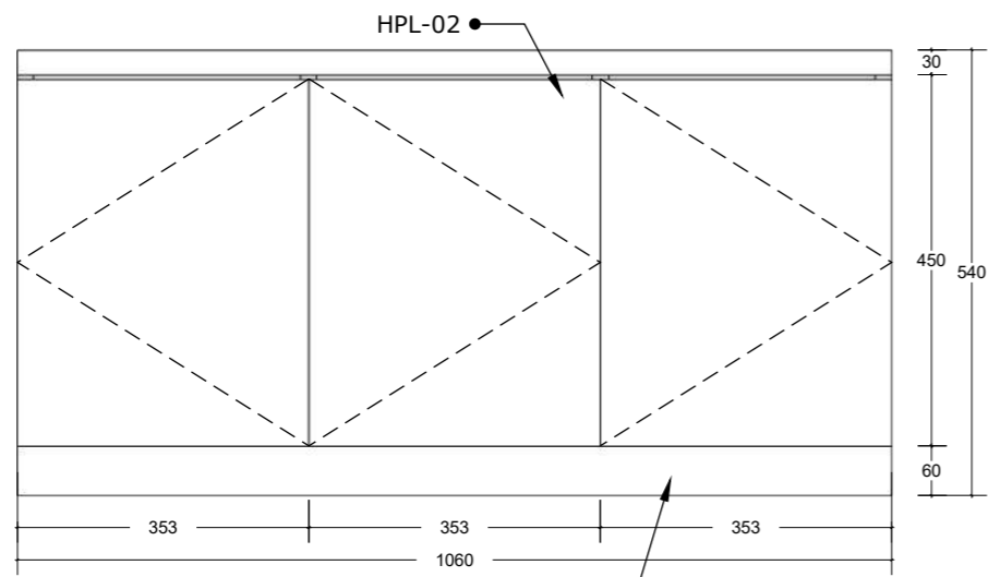
03 FRONT VIEW INT-512 Scale: 1:10
