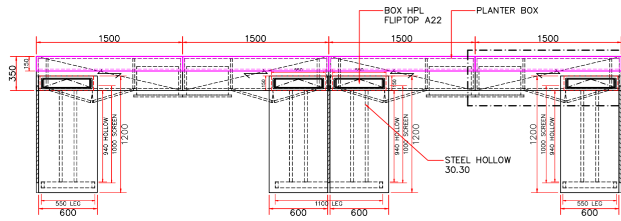
FRONT VIEW INT-517
