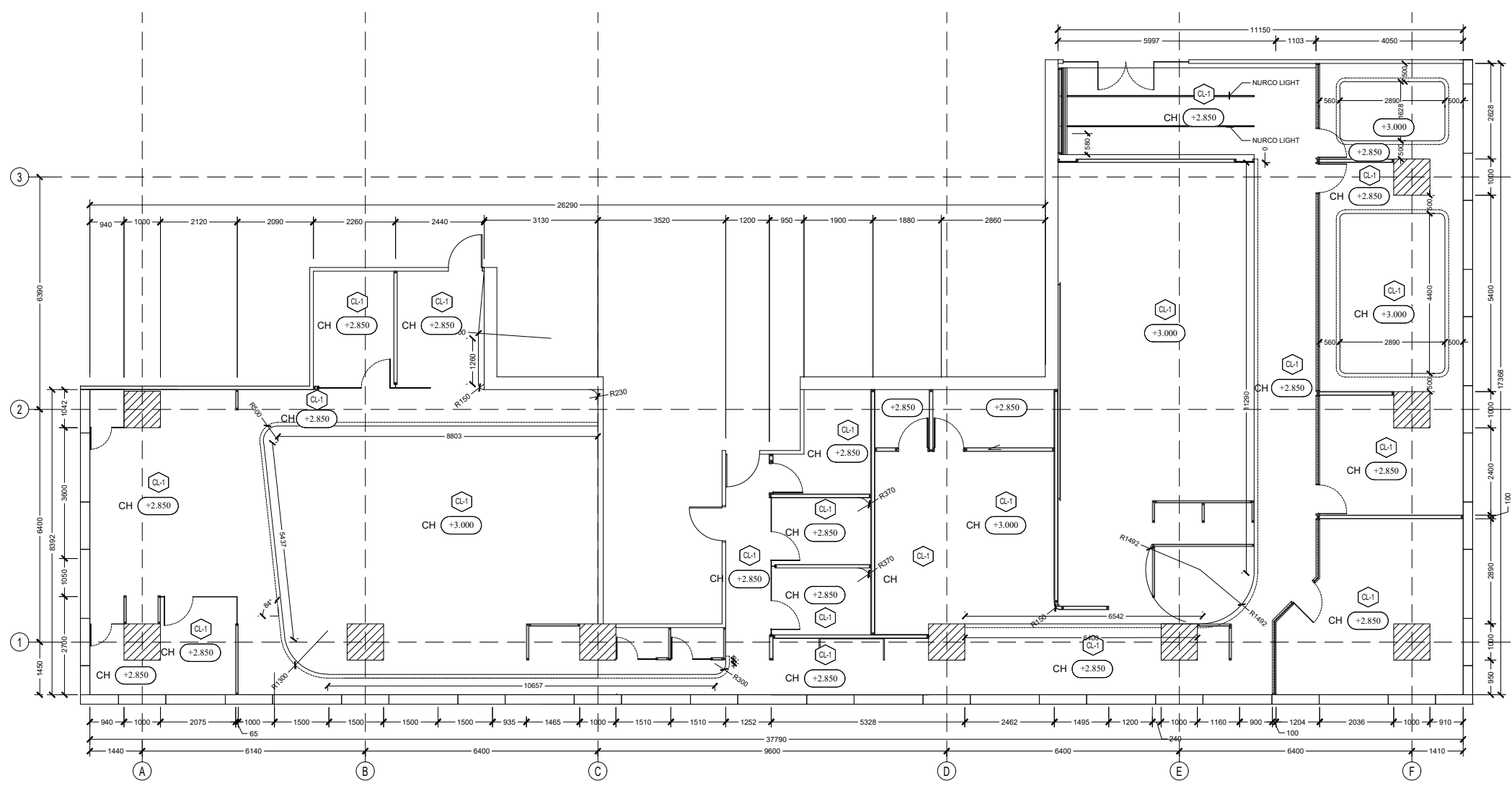
INT-105 CEILING PLAN SCALE 1 : 150
