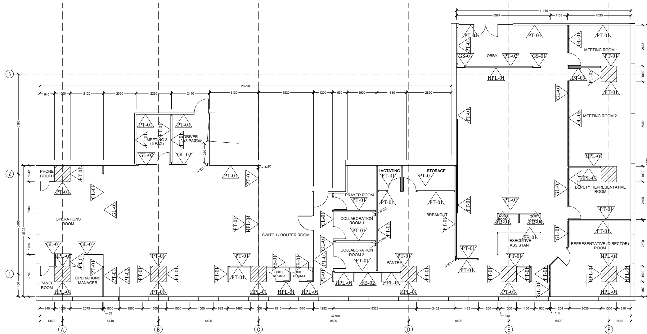
INT-104 WALL FINISHES PLAN SCALE 1 : 150
