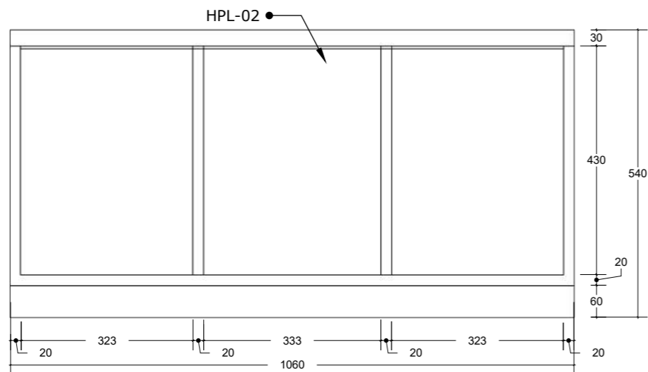
04 FRONT VIEW WITHOUT DOOR INT-512 Scale: 1:10
