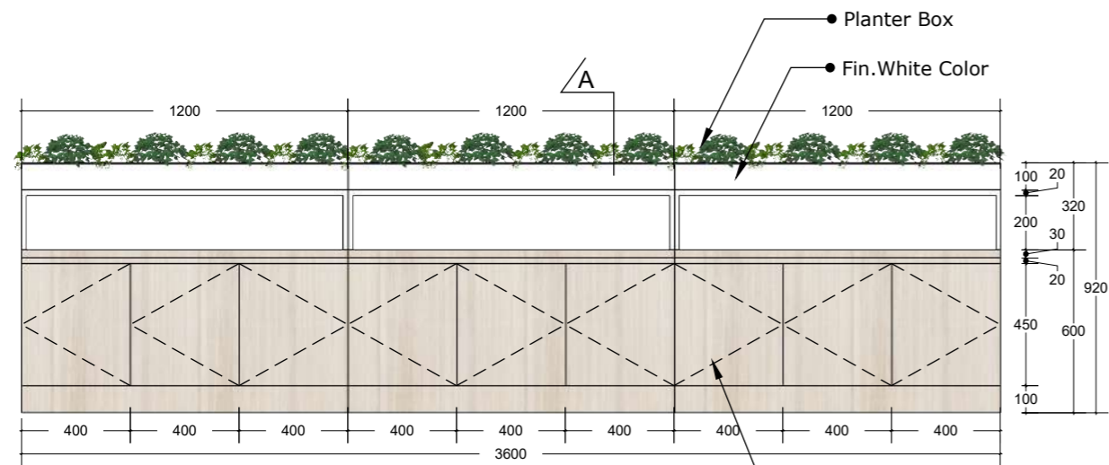
03 FRONT VIEW INT-514 Scale: 1:25
