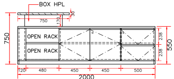
VIEW SIDE CREDENZA
