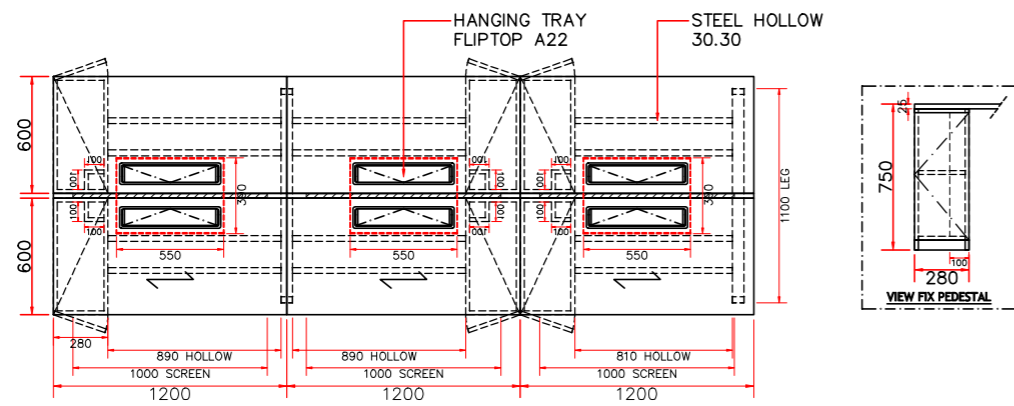
TOP VIEW INT-517
