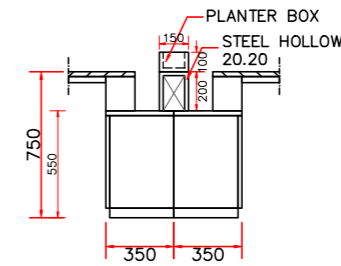
FRONT VIEW SIDE CREDENZA
