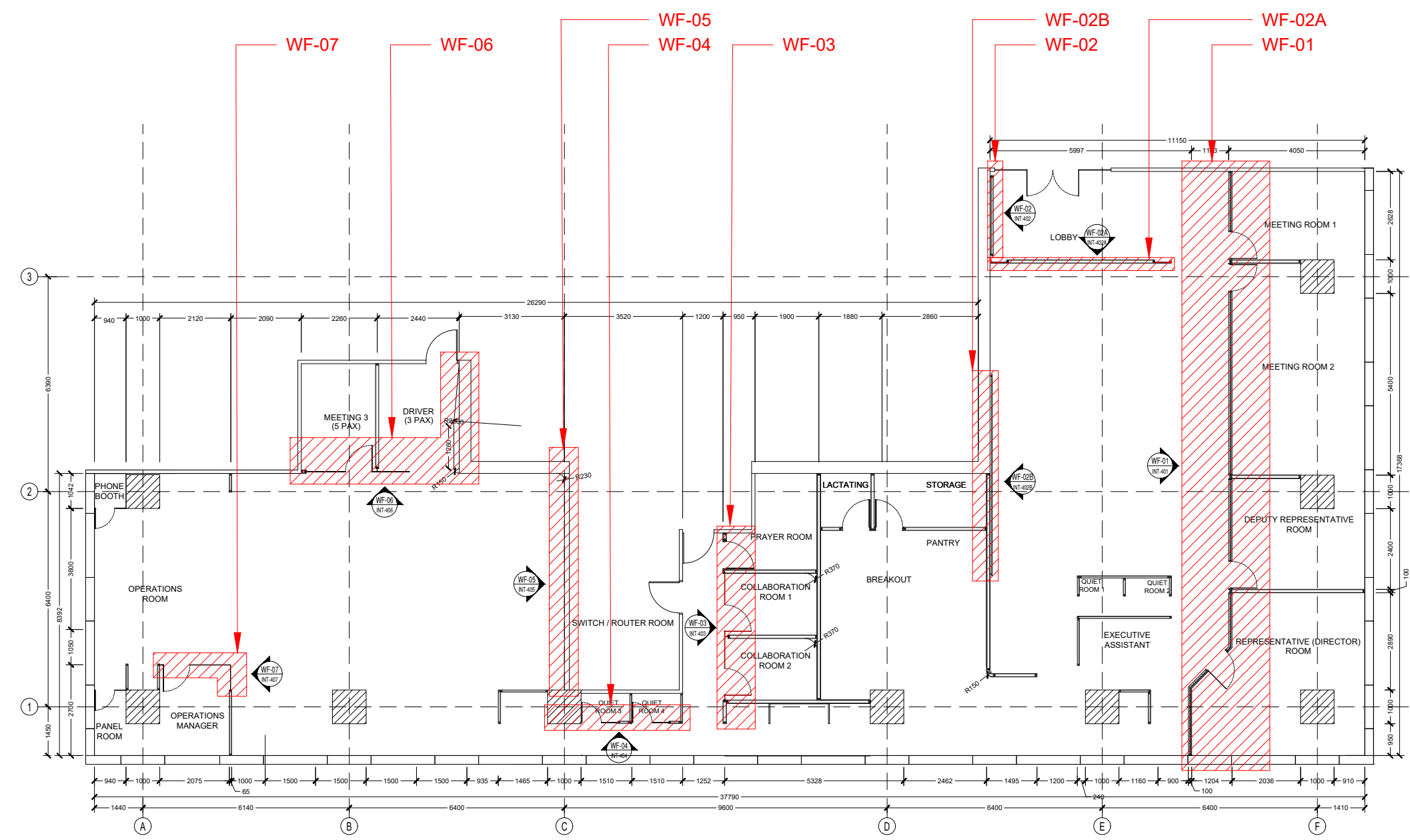
INT-103.A FEATURE WALL PLAN SCALE 1 : 150
